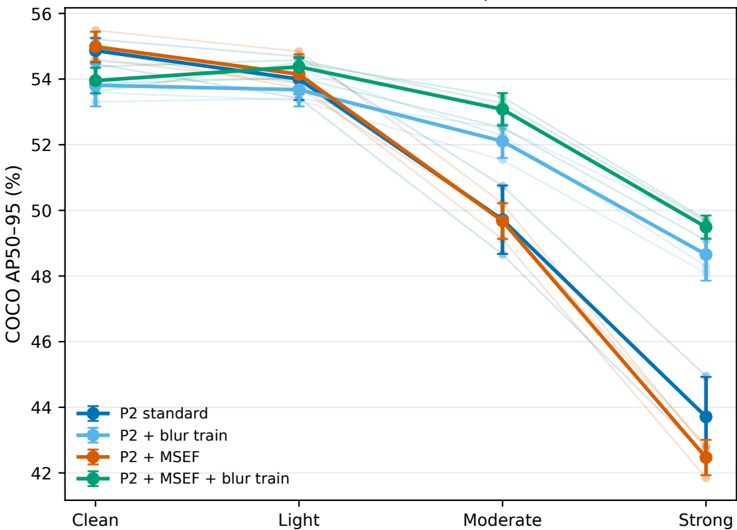
(a) Robustness curve (mean \pm sample SD, n=3 seeds)
