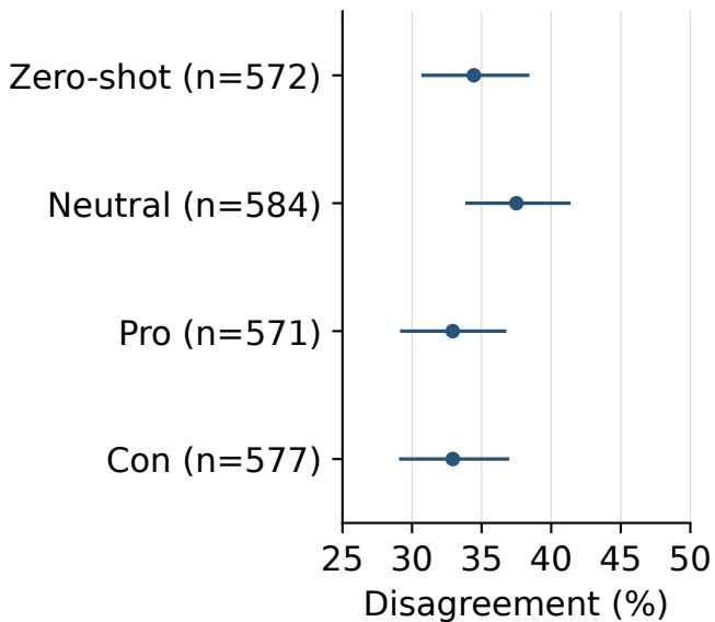
(b) Qwen3 30B
