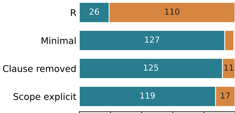
Qwen / Chinese
