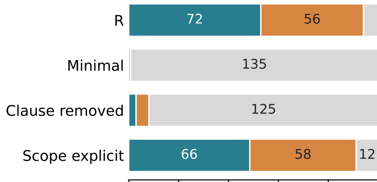
Mistral / Chinese
