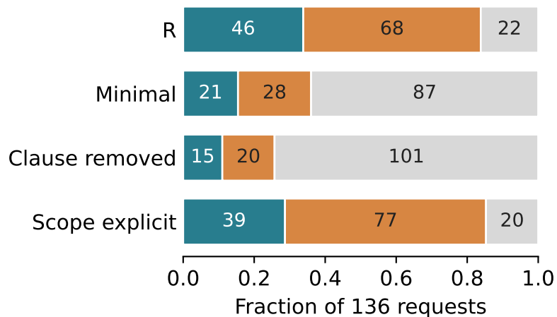
Mistral / Spanish
