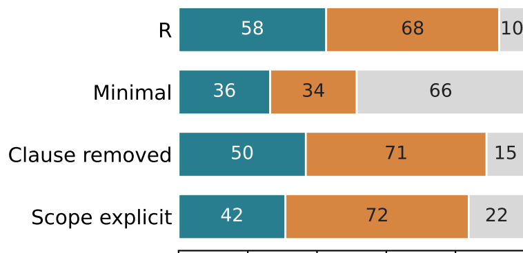
Mistral / Spanish
