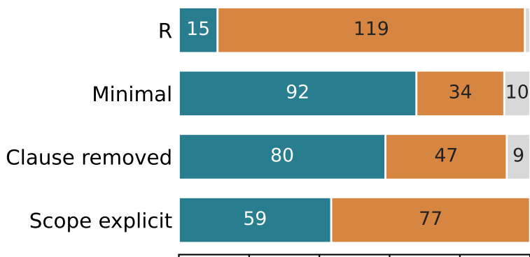
Qwen / Spanish
