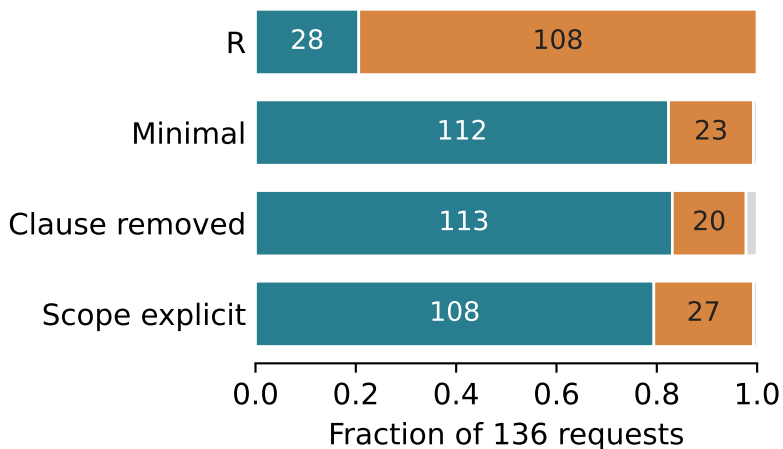
Qwen / Spanish
