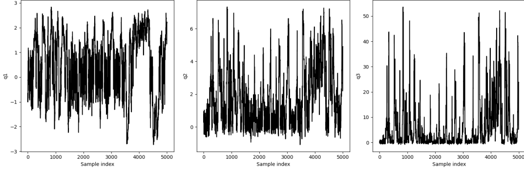
Figure 3: Degeneracy in sampling when using L-HNNs in NUTS for a 3-D Rosenbrock density. These trace plots correspond to the three dimensions q_1 , q_2 , and q_3 .
