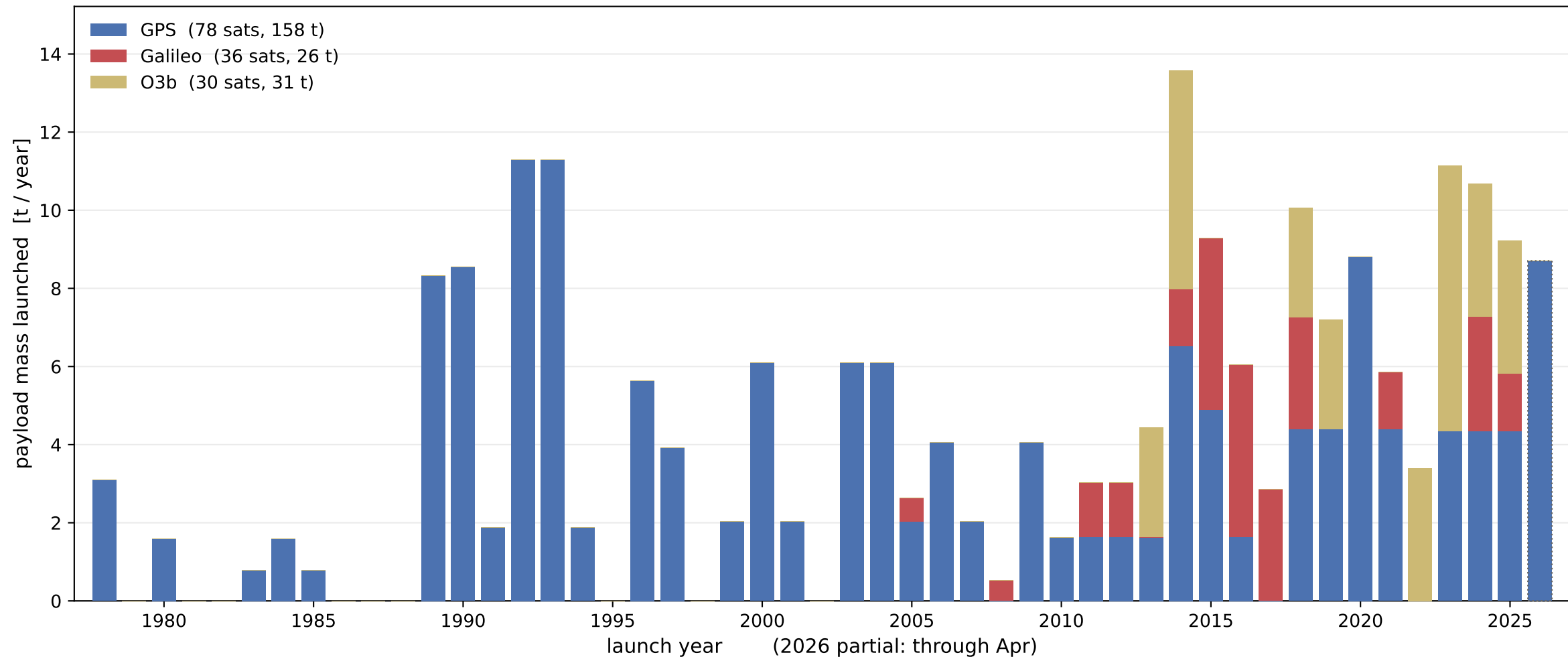
GPS, Galileo and O3b: payload mass launched per year, 1978-2026
