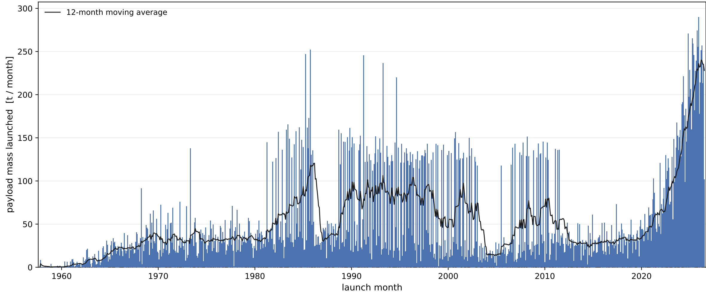
Payload mass launched to orbit per month, 1957-2026
