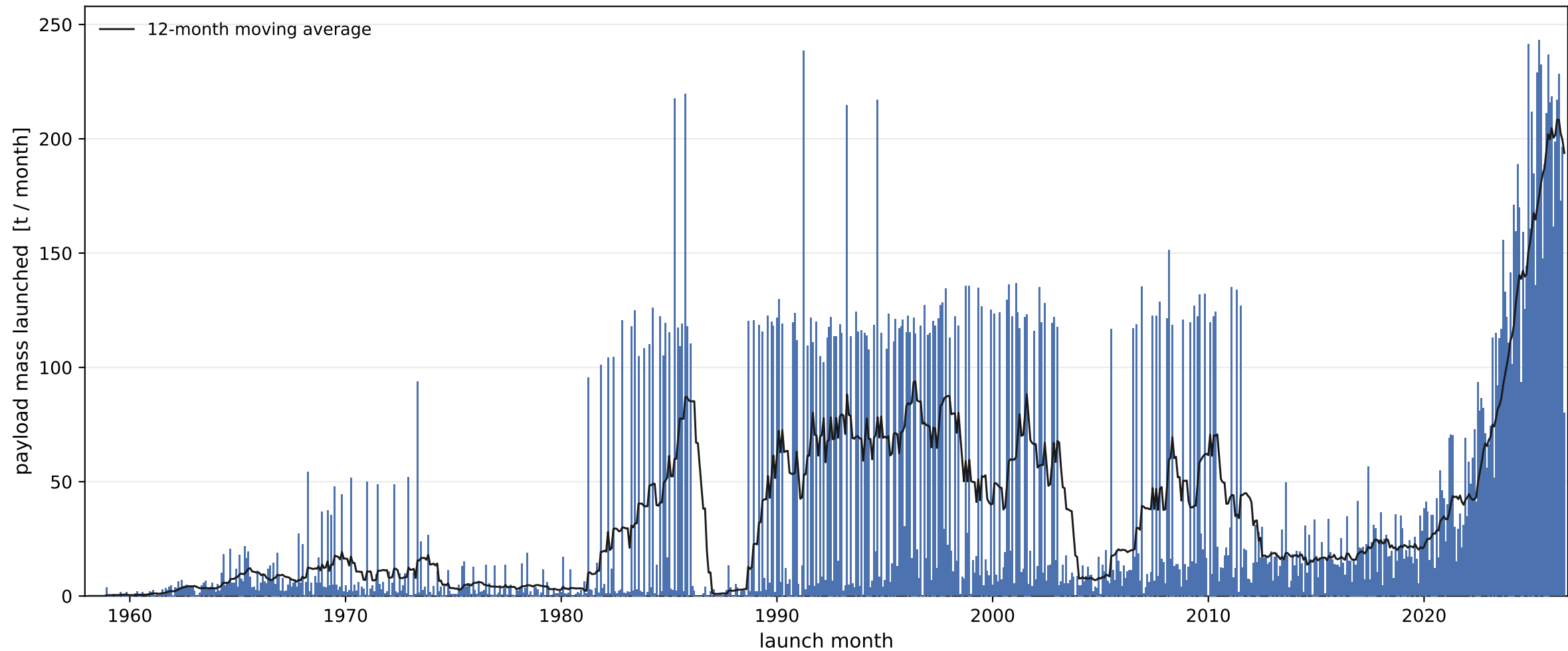
Payload mass launched to orbit per month, 1958-2026 (excluding Chinese, Russian and Soviet satellites)
