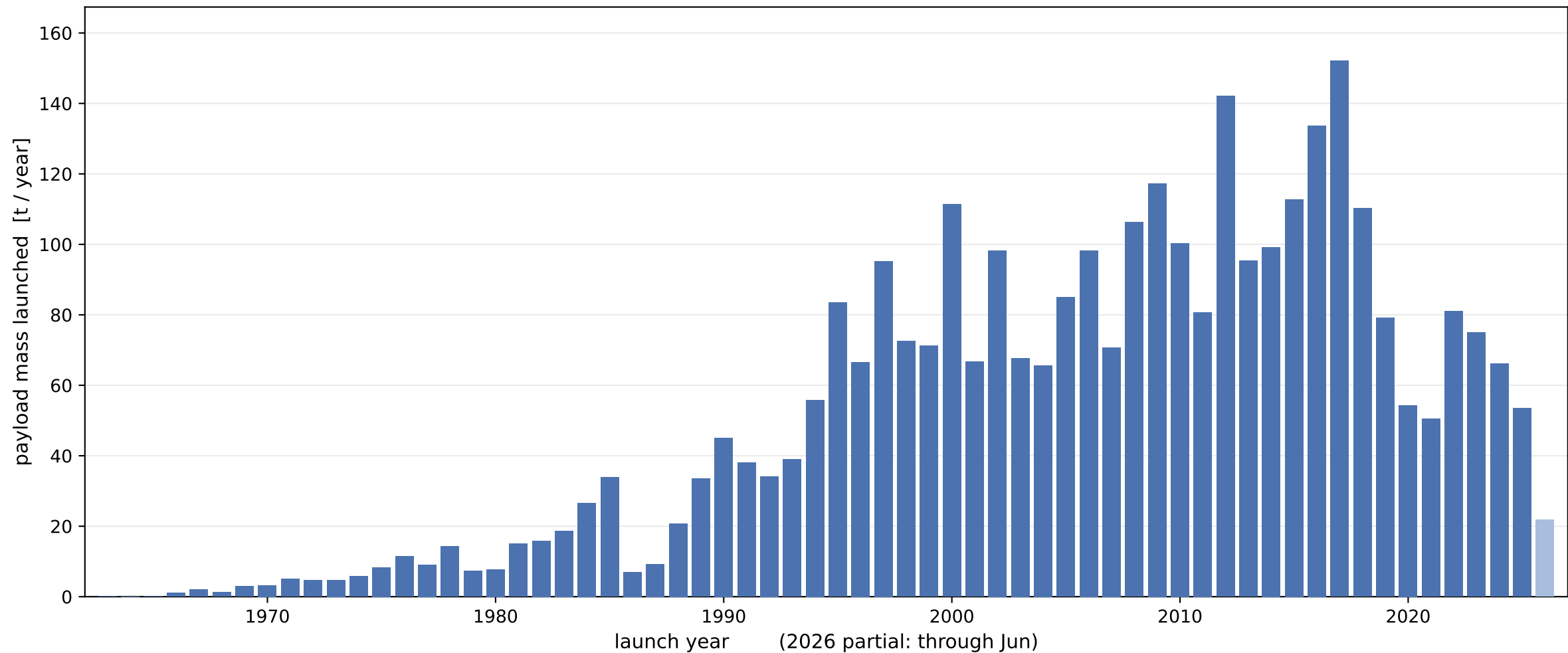
Payload mass launched to orbit per year, 1963-2026 (GEO-bound only; CN/RU/SU satellites excluded)
