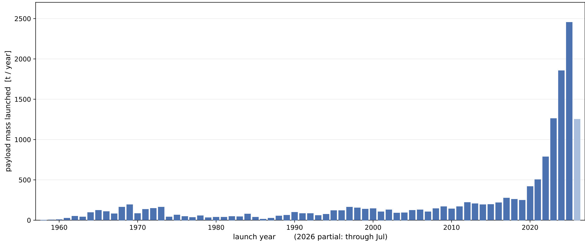
Payload mass launched to orbit per year, 1958-2026 (Shuttle orbiters excluded; CN/RU/SU satellites excluded)
