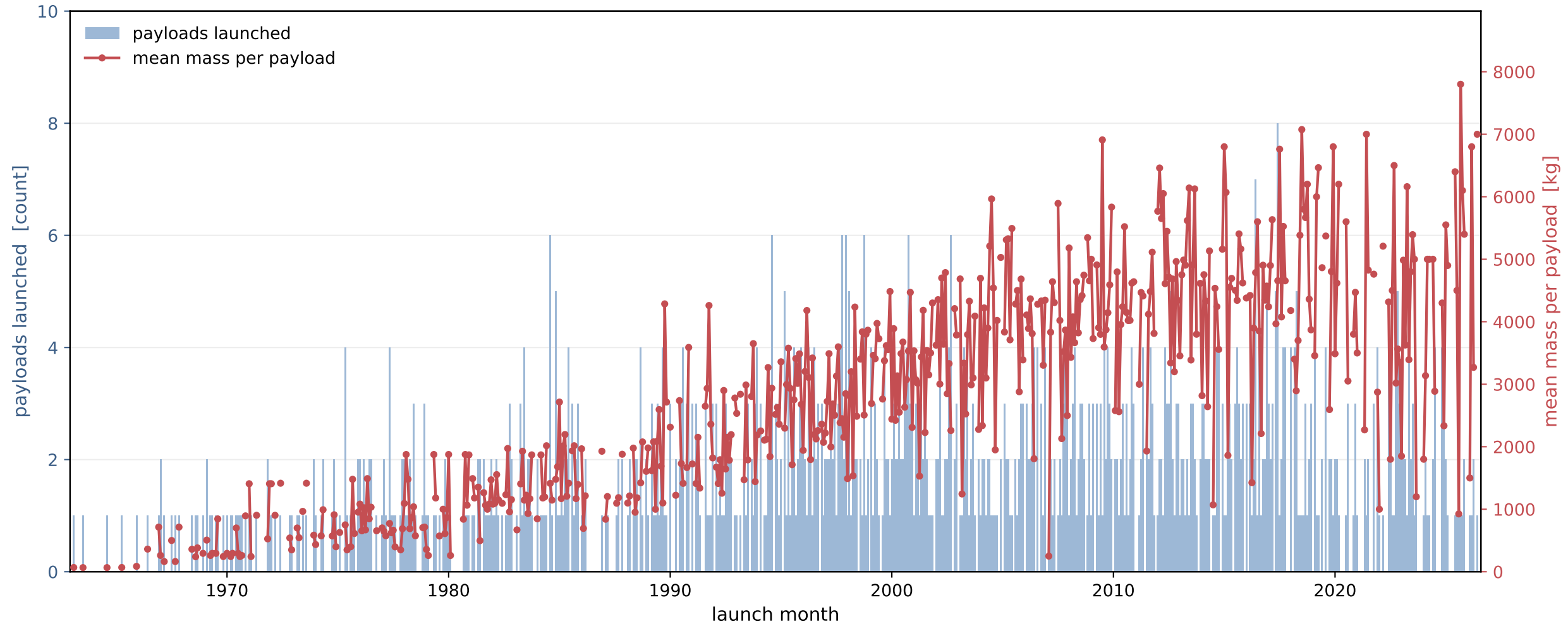
GEO payloads: count and mean mass per month, 1963–2026
