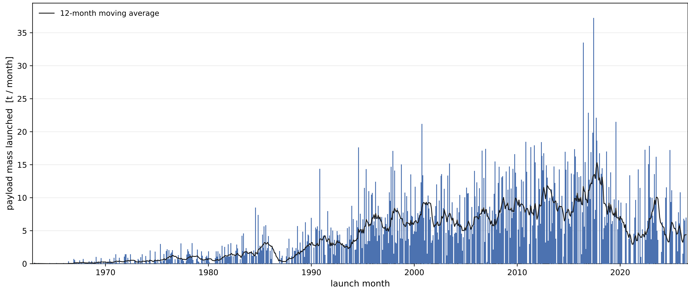
Payload mass launched to orbit per month, 1963–2026
