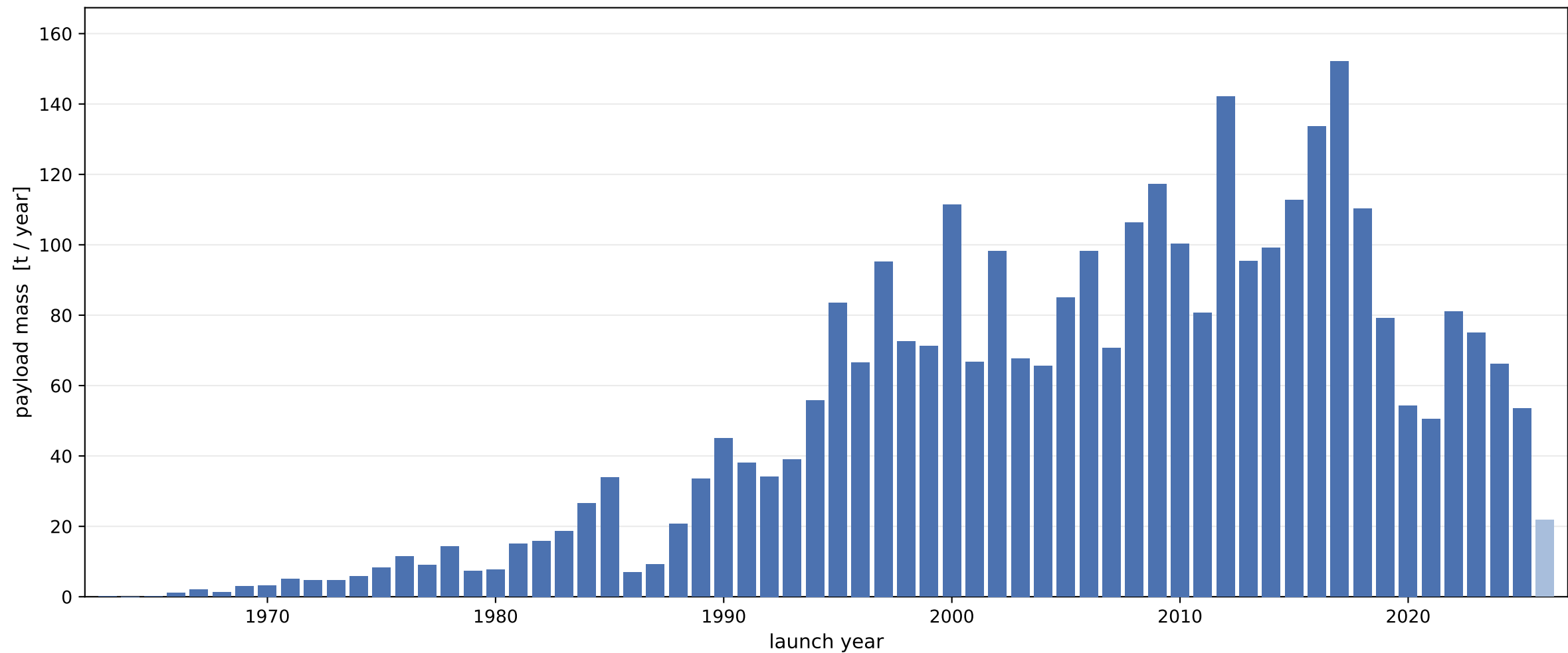
Payload mass launched to orbit per year, 1963-2026
