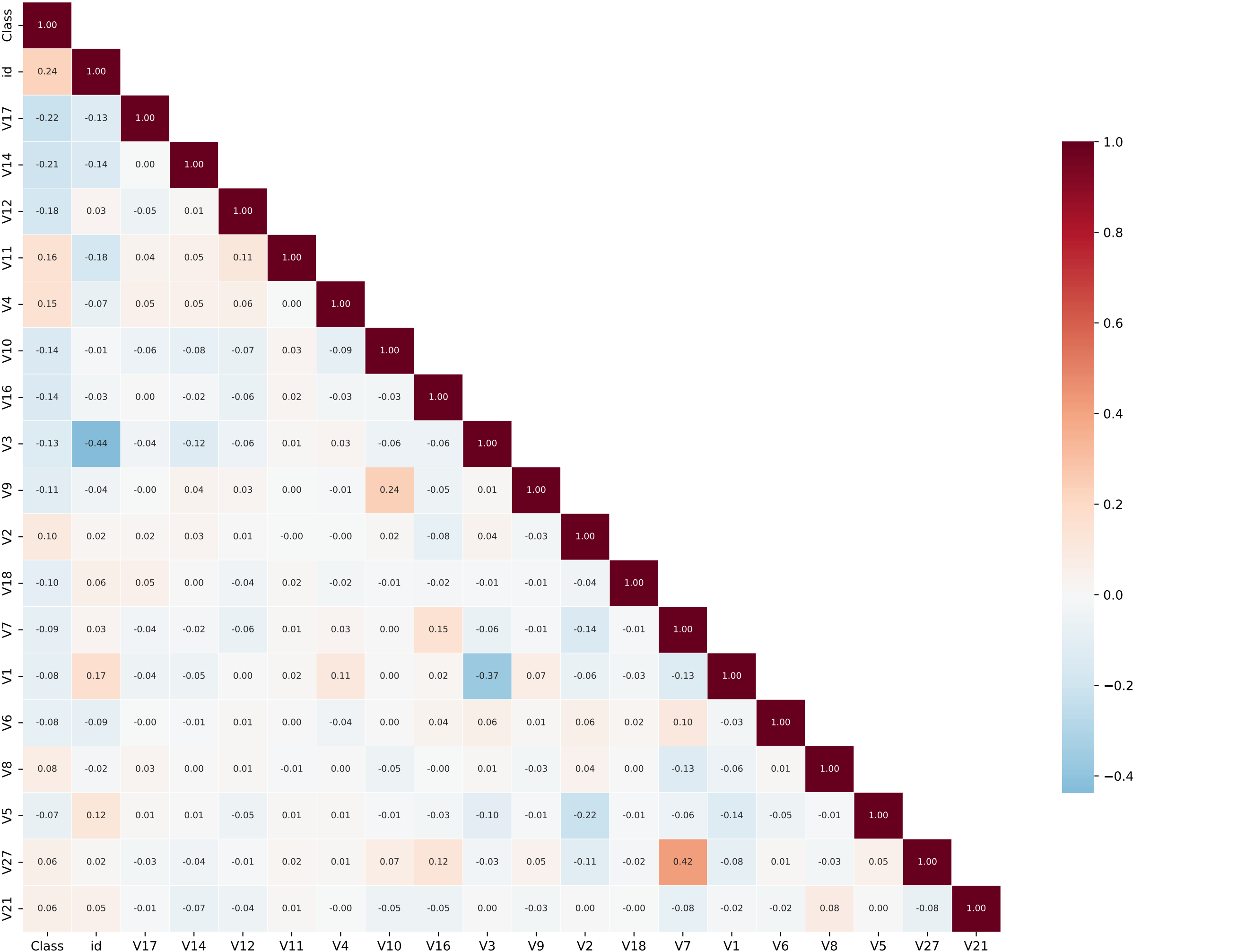
Feature Correlation Heatmap (Top-20 features by |corr| with Class)
