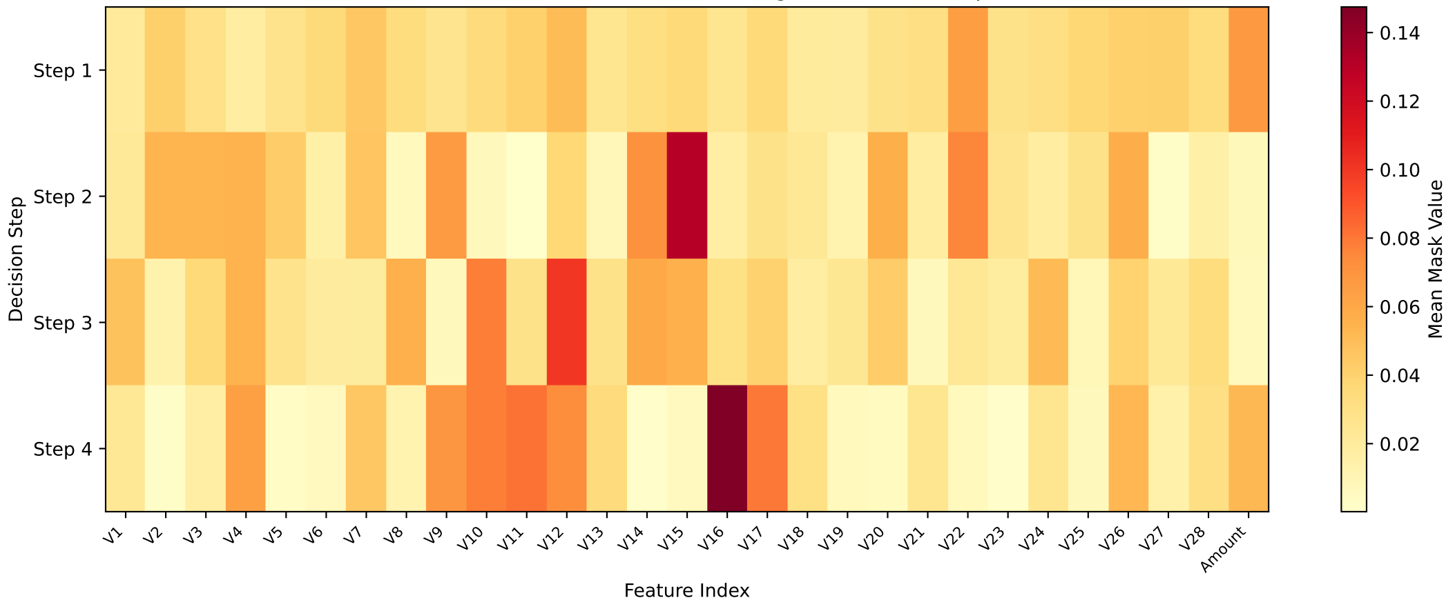
TabNet Feature Selection Masks (averaged over 500 samples)
