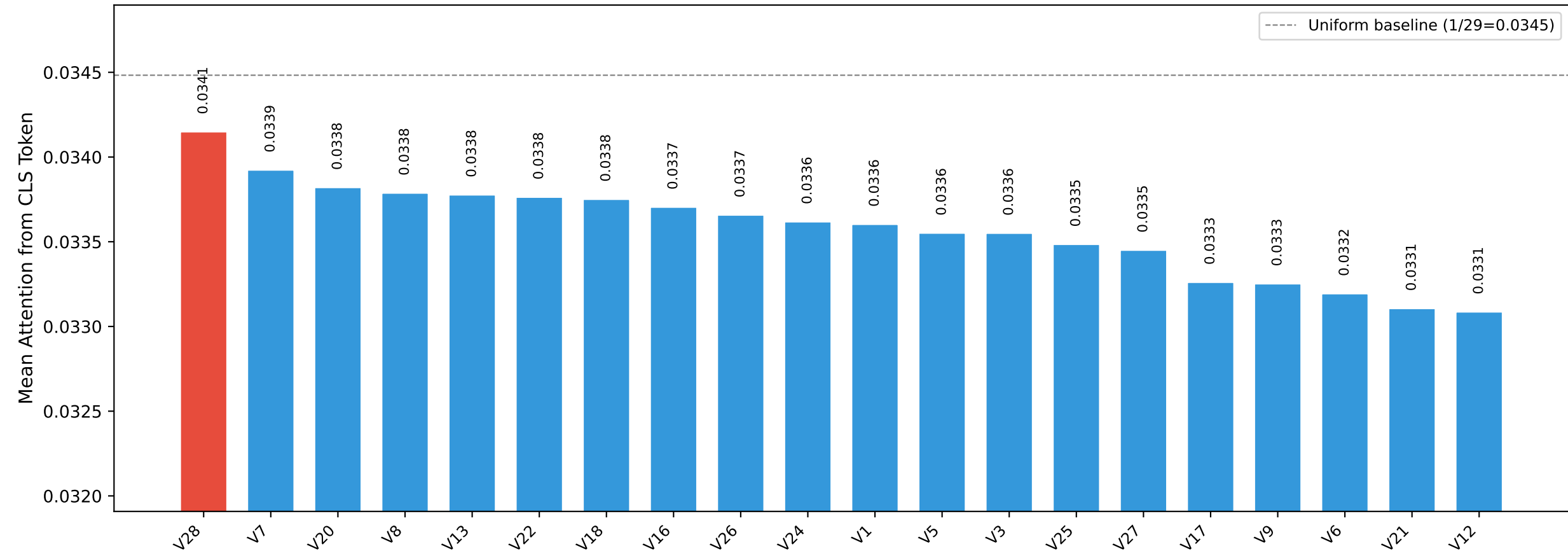
FT-Transformer: CLS Attention to Feature Tokens (Top-20) | Mean=0.0334 Range=[0.0327, 0.0341] Std=0.00038
