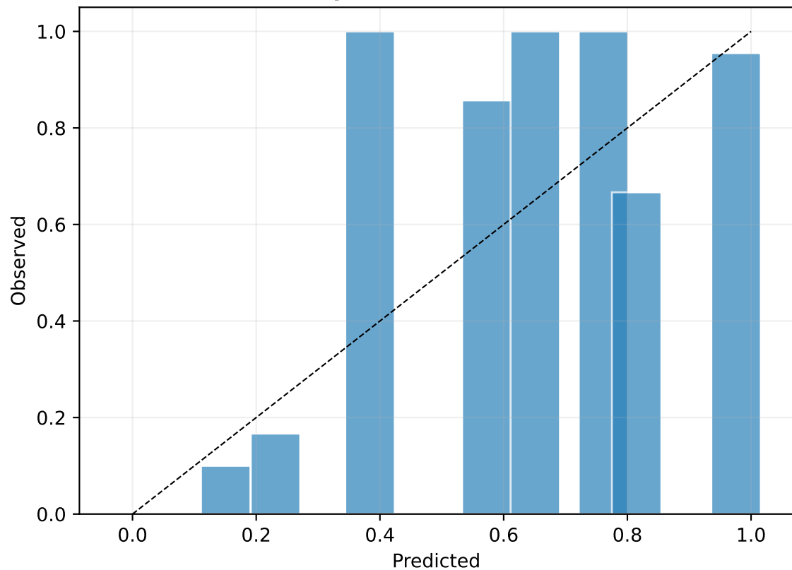
FTT+Sparsemax (ECE=0.0067)
