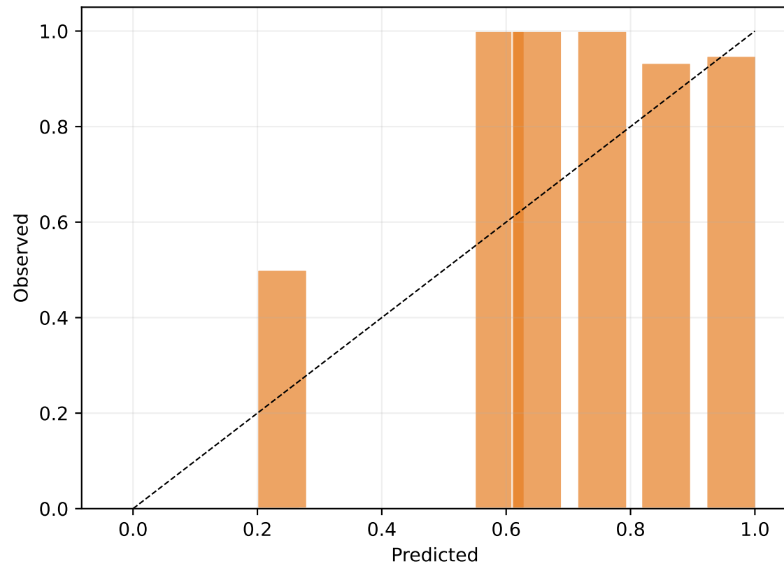
FTT+Softmax (ECE=0.0091)
