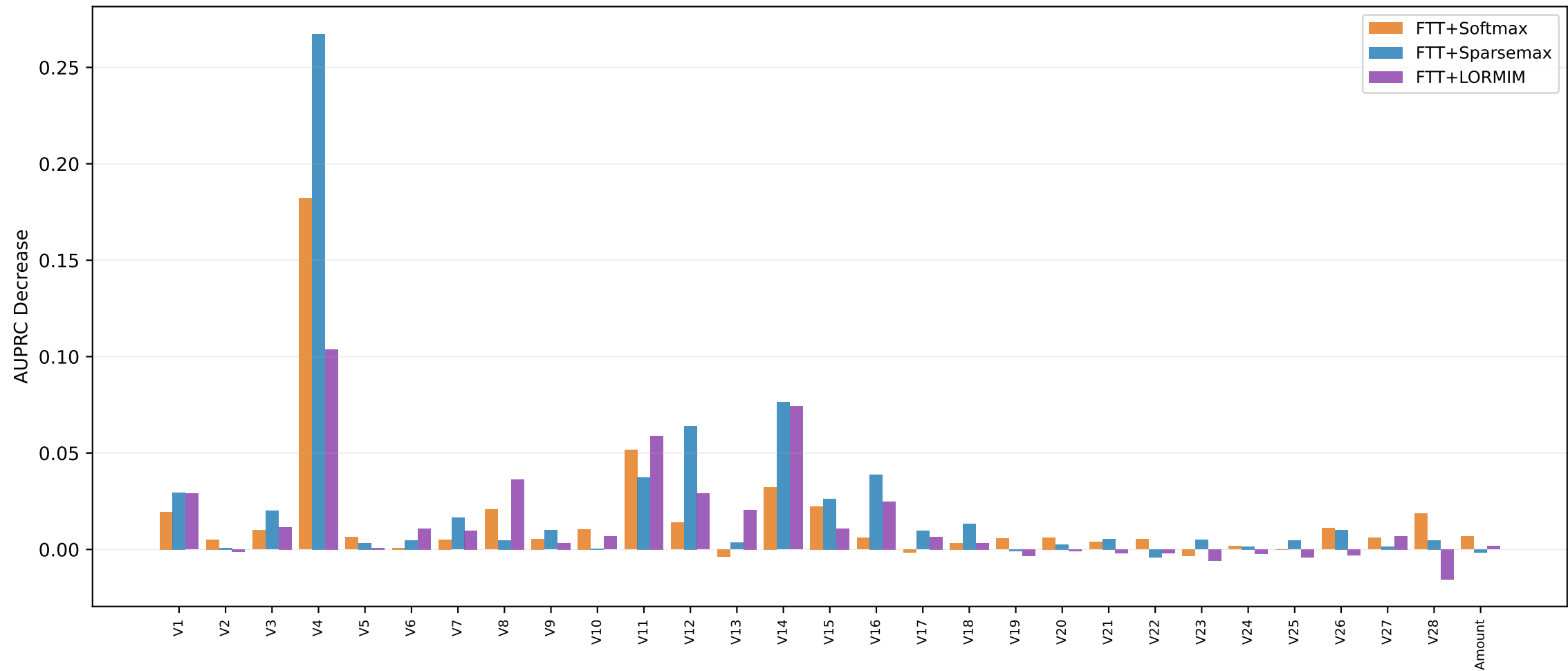
Permutation Importance ( r(\text{Soft}, \text{Sparse})=0.946 , r(\text{Soft}, \text{LORMIM})=0.806 )
