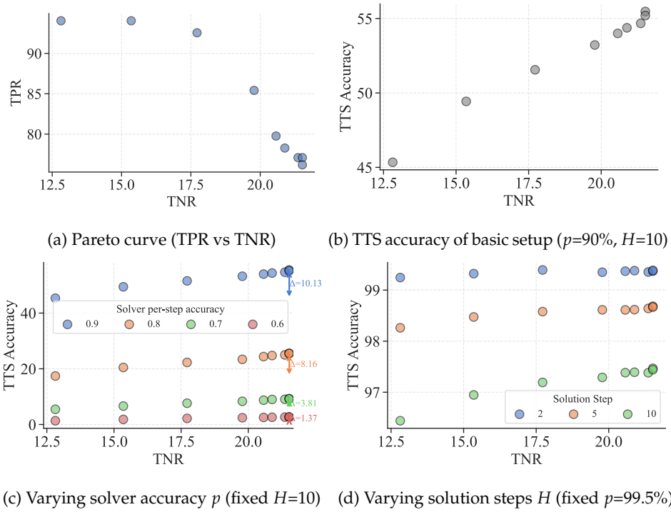
Figure 6: Pareto curve of TPR vs. TNR and its impacts on performance of test-time scaling (TTS) method, localized rejection sampling. Results shown for Qwen3-8B-thinking on Hard2Verify. (a) Varying the sample-level threshold \tau produces large drop alongside an increase in TNR. (b) Simulated TTS accuracy under the basic setup ( p = 90\% , H = 10 ): accuracy increases steadily as the verifier is steered toward higher TNR, despite the simultaneous drop in TPR. (c) Higher TNR yields higher TTS accuracy across all solver accuracy levels. (d) Higher TNR is slightly less beneficial when the solution is short ( H=2 ) and solver accuracy is high; otherwise it consistently improves accuracy.
