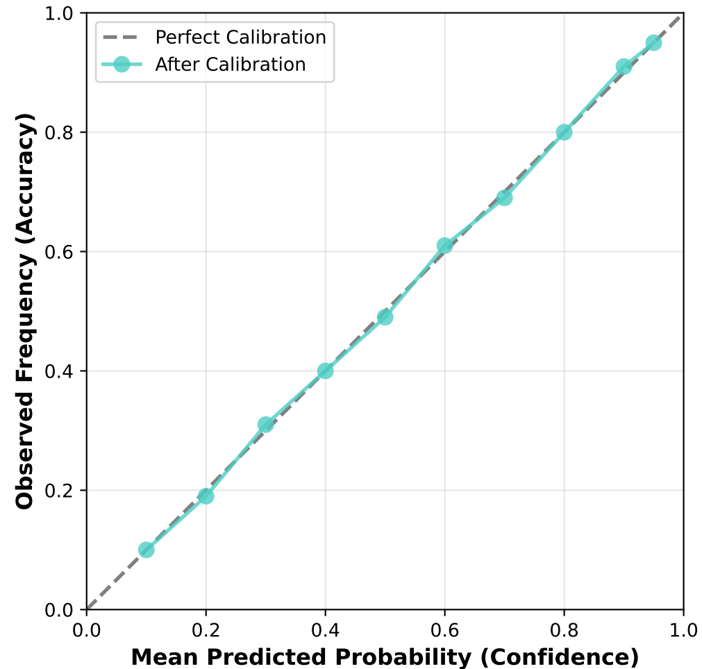
After Isotonic Calibration ECE = 0.028
