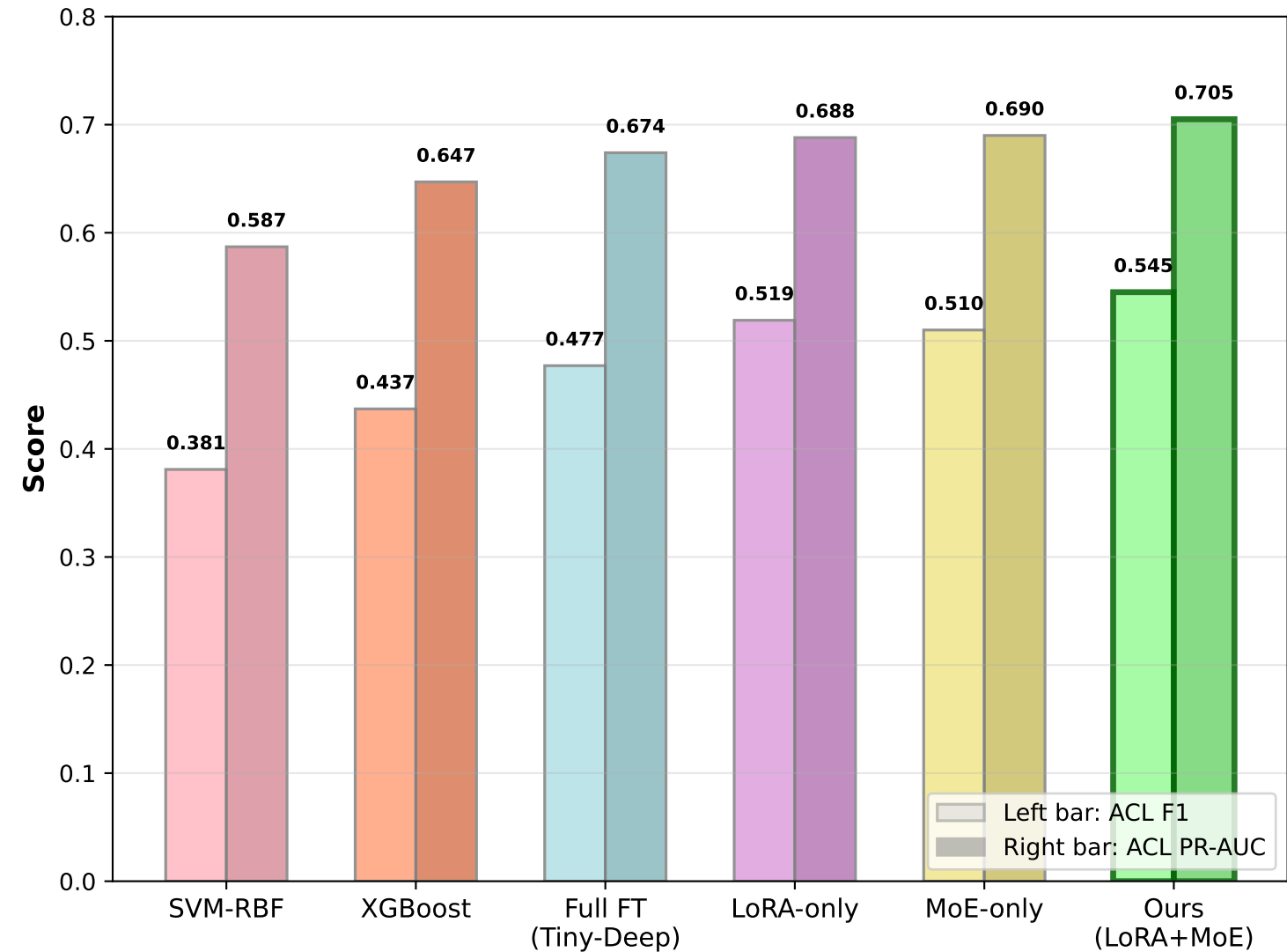
Affective-Cognitive Load (ACL) Classification Performance (Physiology Contribution)
