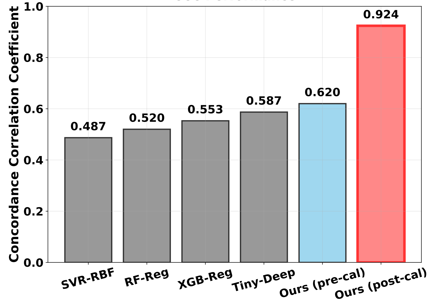
PFI Regression Performance Comparison MAE Performance CCC Performance
