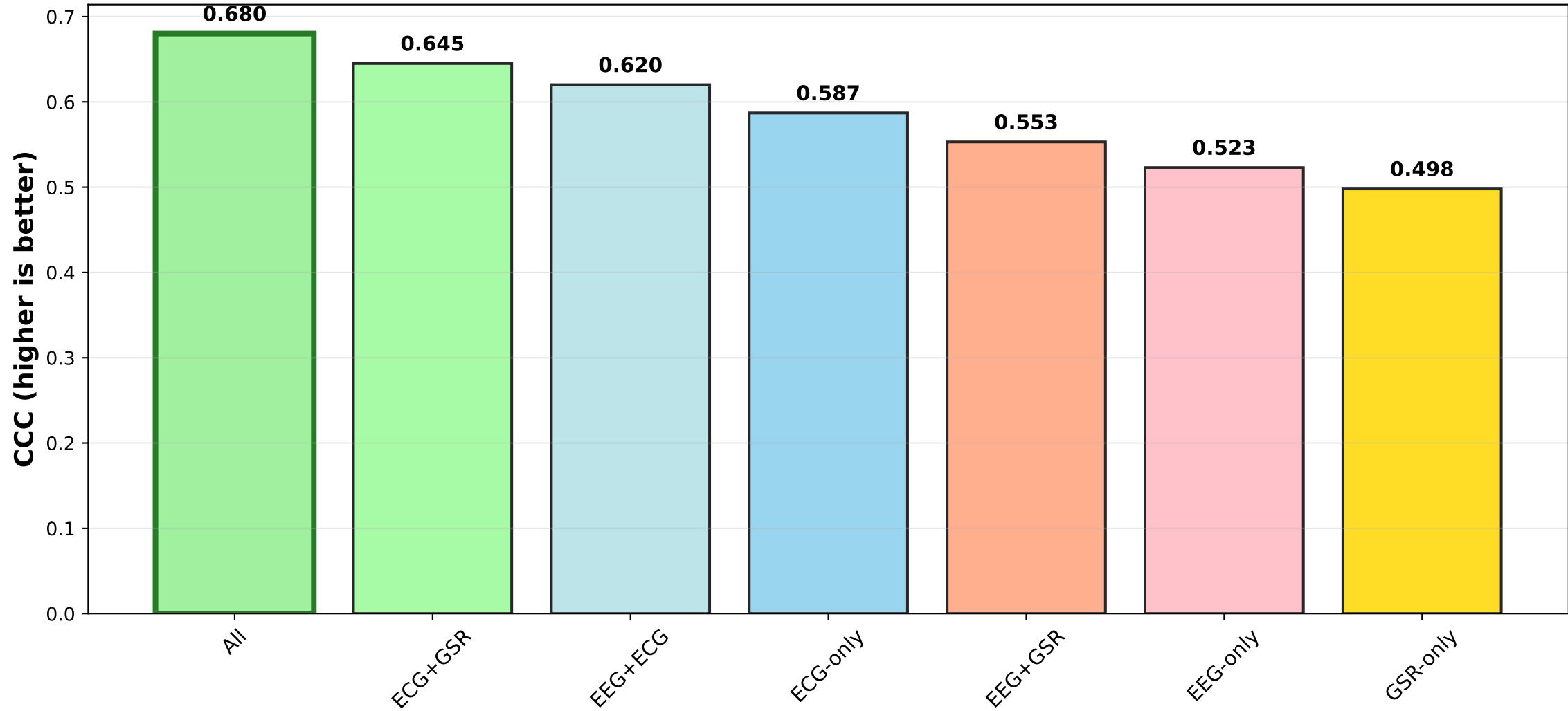
PFI Regression: Modality Contributions (Sorted by CCC)
