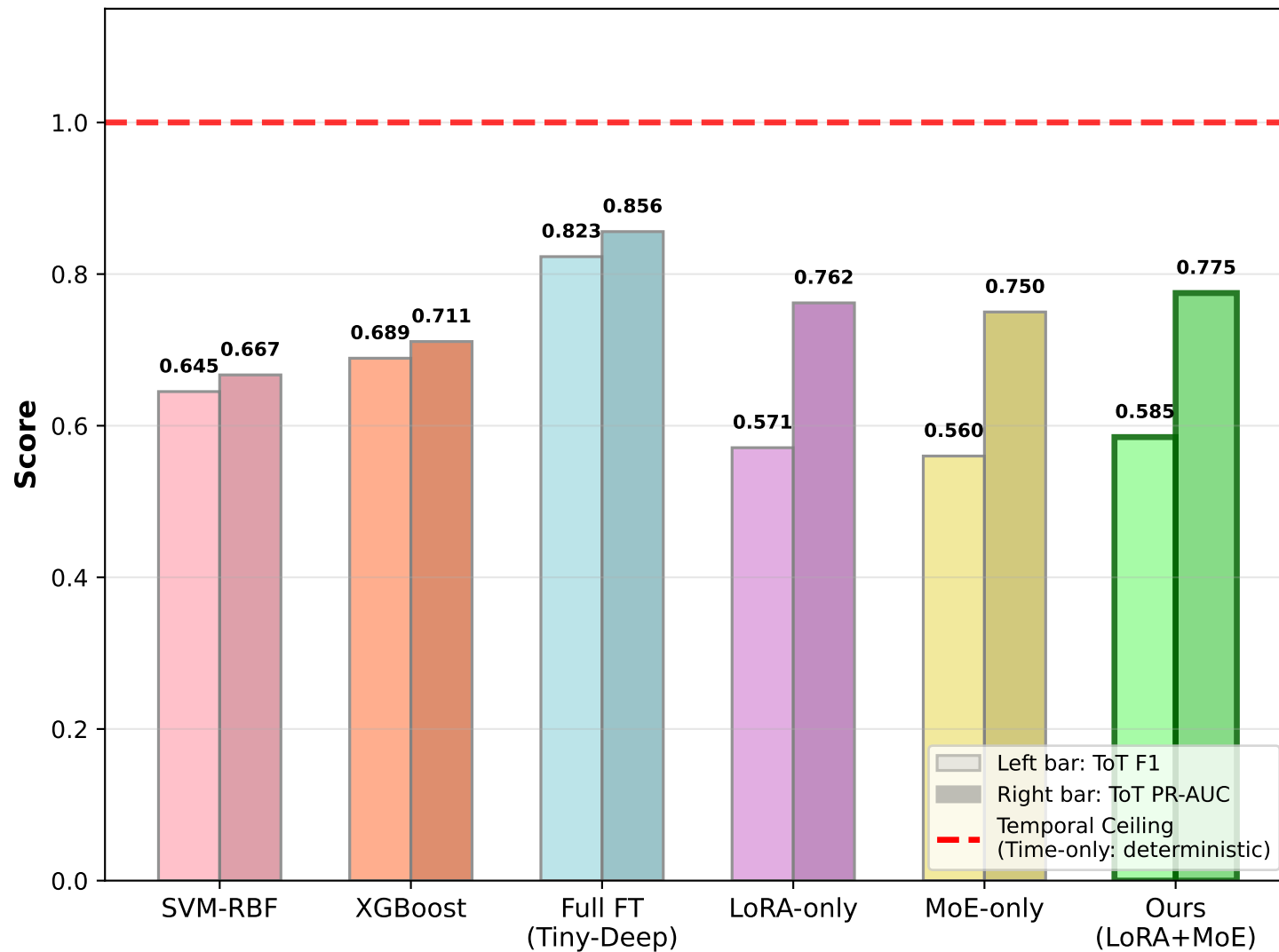
Time-on-Task (ToT) Classification Performance
