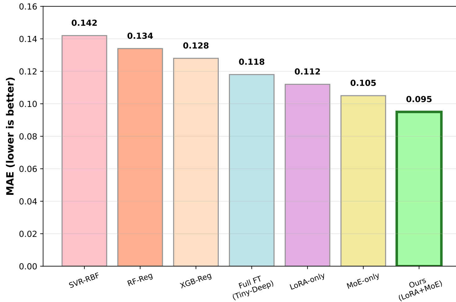
Mean Absolute Error
