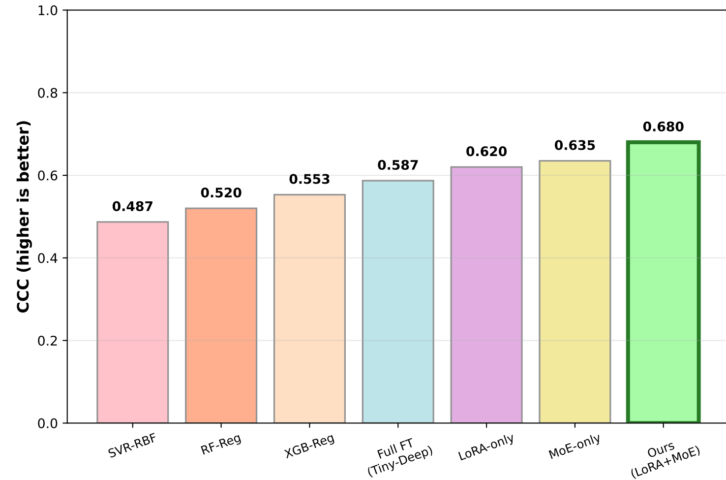
Concordance Correlation Coefficient
