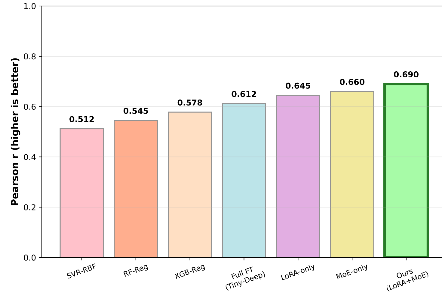
Pearson Correlation Coefficient
