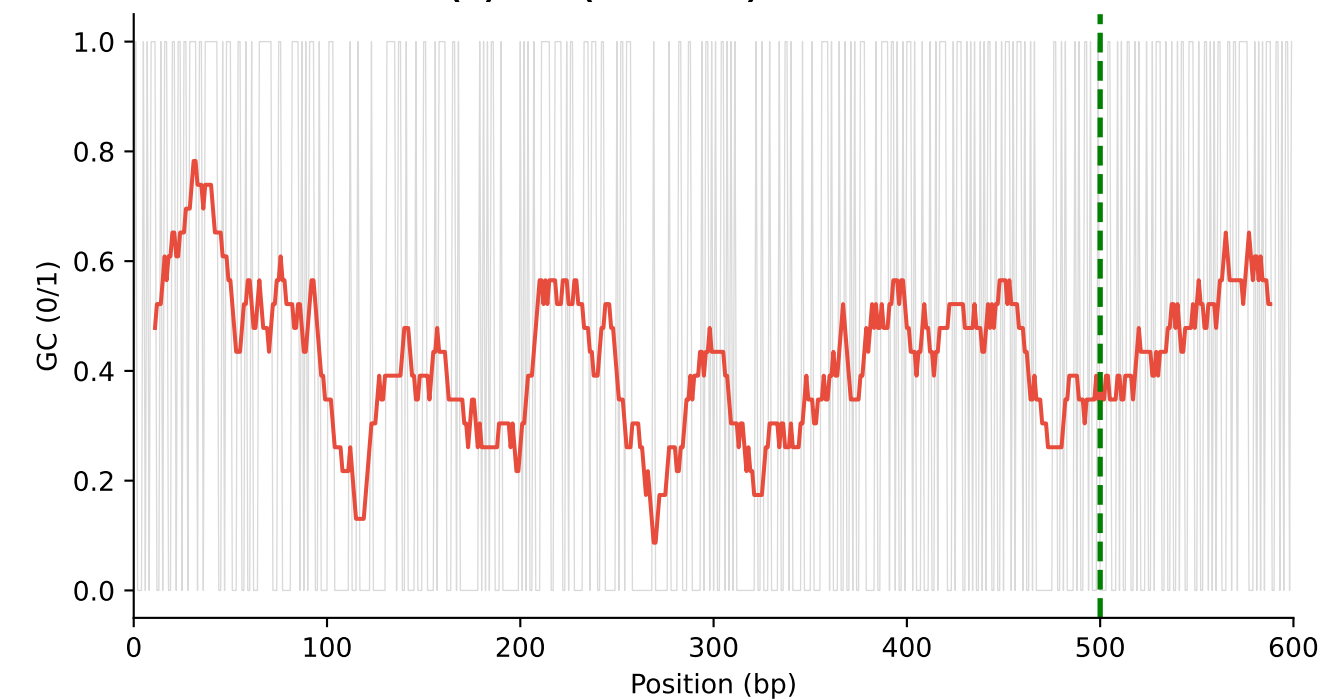
(C) TBP (TATA-box) - GC Content
