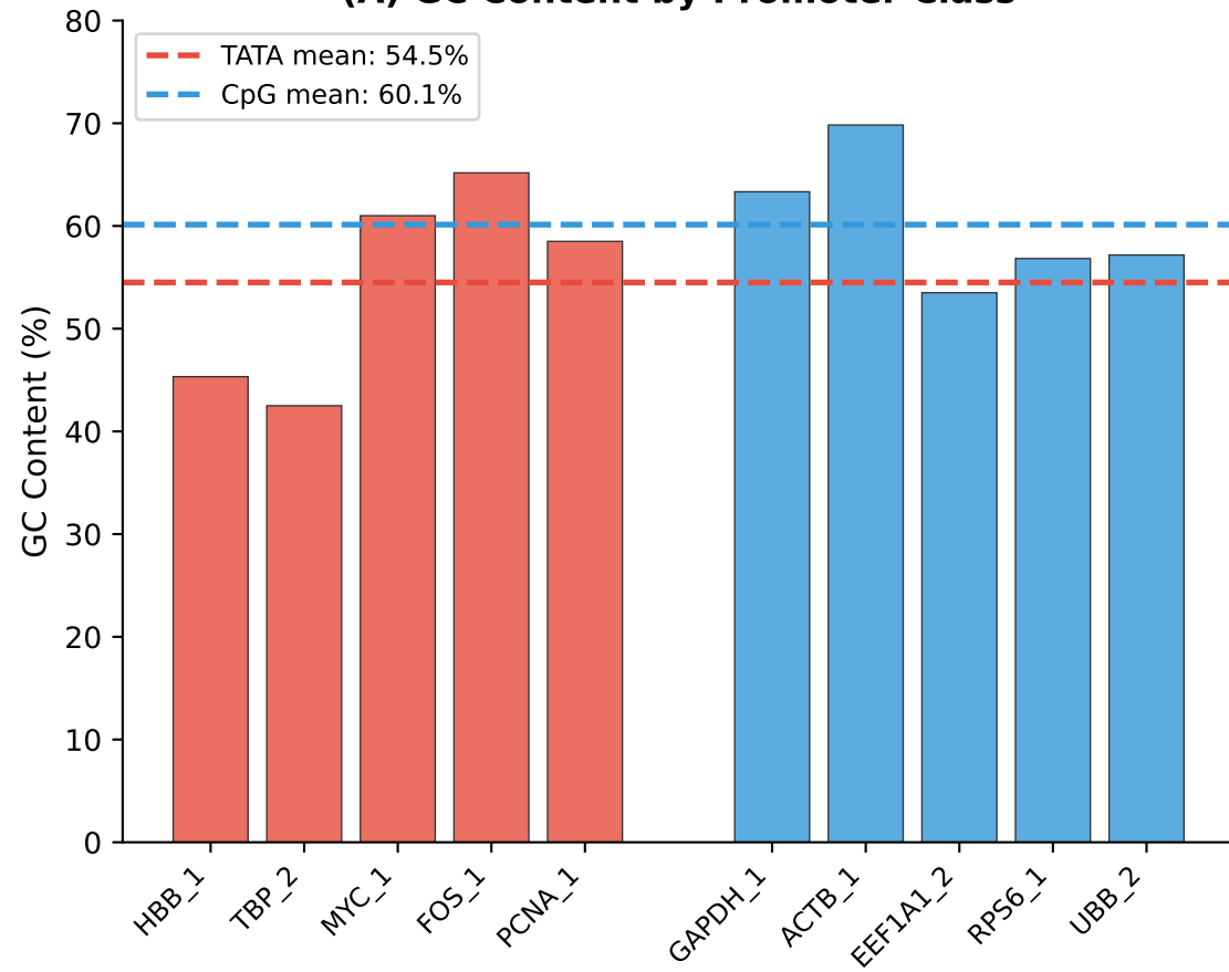
(A) GC Content by Promoter Class
