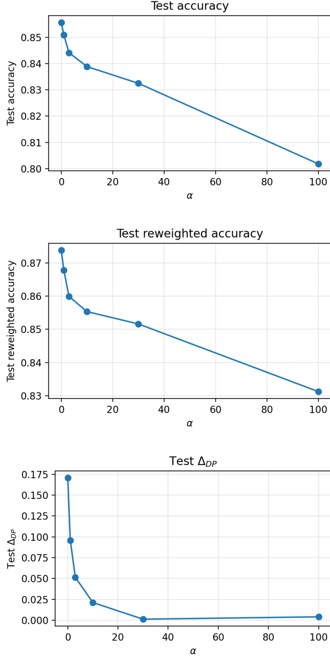
Figure 1: Test accuracy, reweighted accuracy, and \Delta_{DP} versus \alpha .
