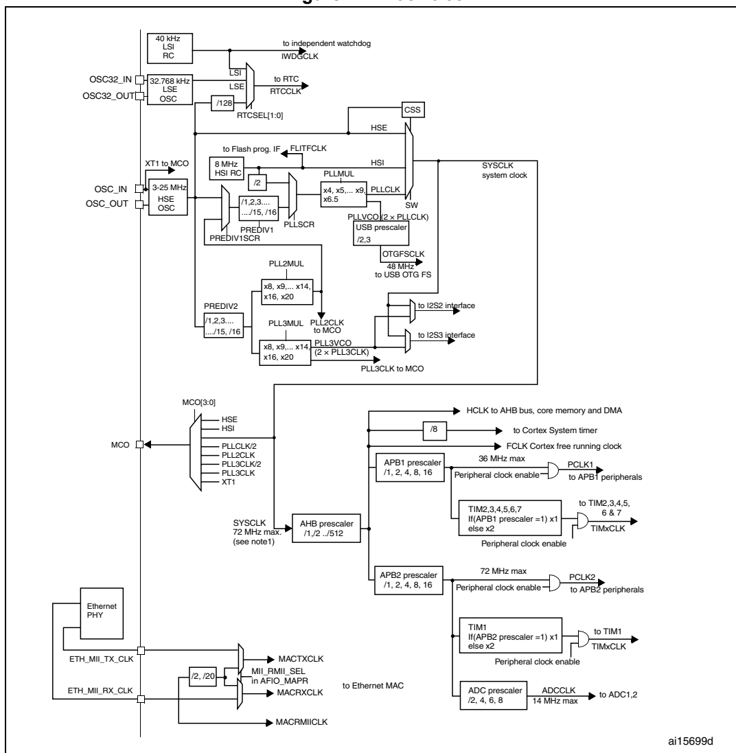
Figure 11. Clock tree
