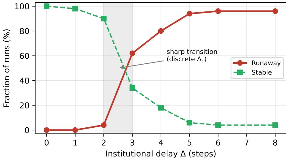
Reactive agents: stable baseline destabilized by delay ( k = 10 , N = 240 , 50 seeds/cell)
