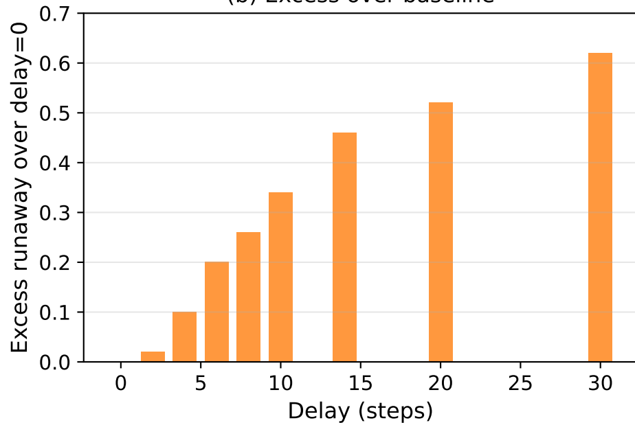
(b) Excess over baseline
