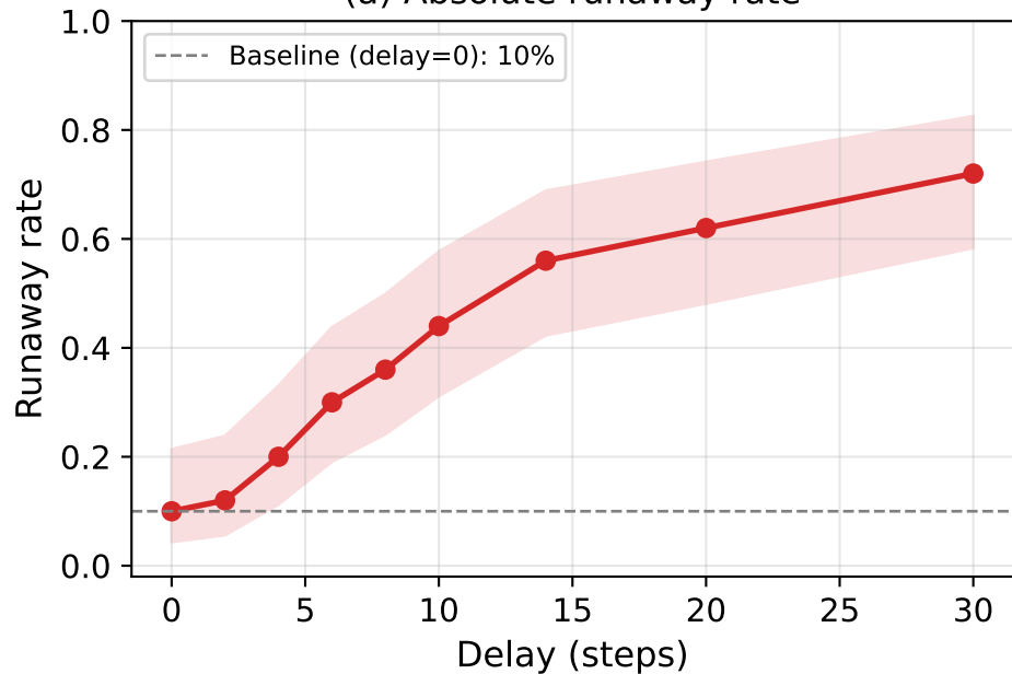
(a) Absolute runaway rate
