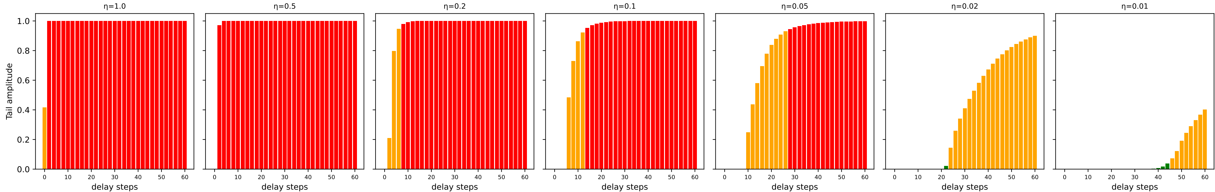
Discrete Mean-Field: \eta controls effective stability margin Green=stable, Orange=oscillatory, Red=runaway
