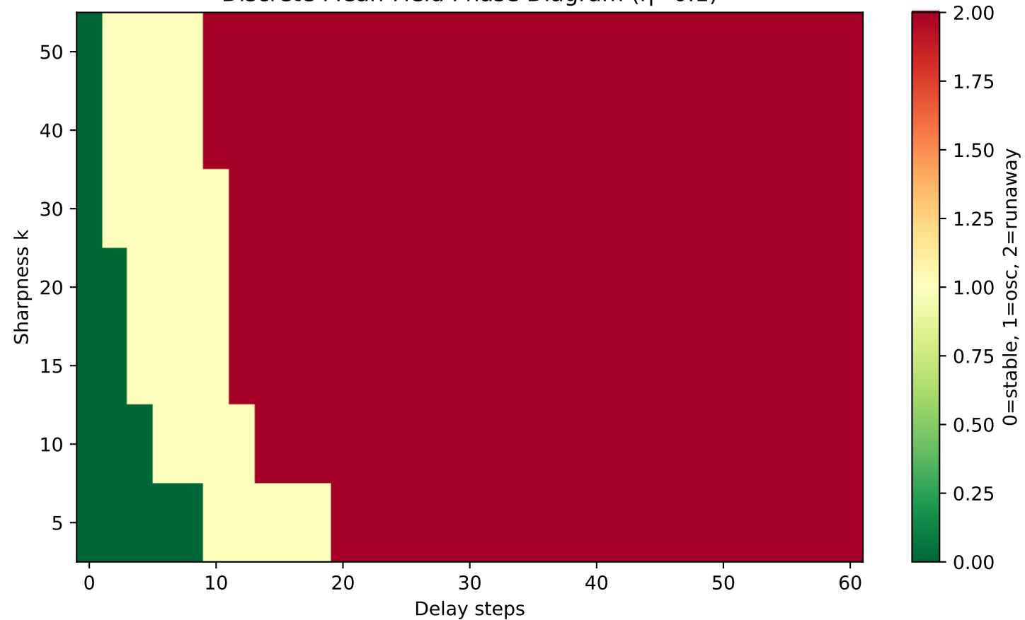
Discrete Mean-Field Phase Diagram ( \eta=0.1 )
