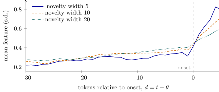
Figure 3: The novelty windows on the same onset alignment, in standardized units. They drift up before the onset (the width-20 window by +0.126 over the last 30 faithful tokens) and then rise +0.195 more in the five tokens after it. The pre-onset climb is what a forecaster can use; the post-onset jump, several times larger, is what a detector sees. The asymmetry is why forecasting scores below detection on the same feature stream.
