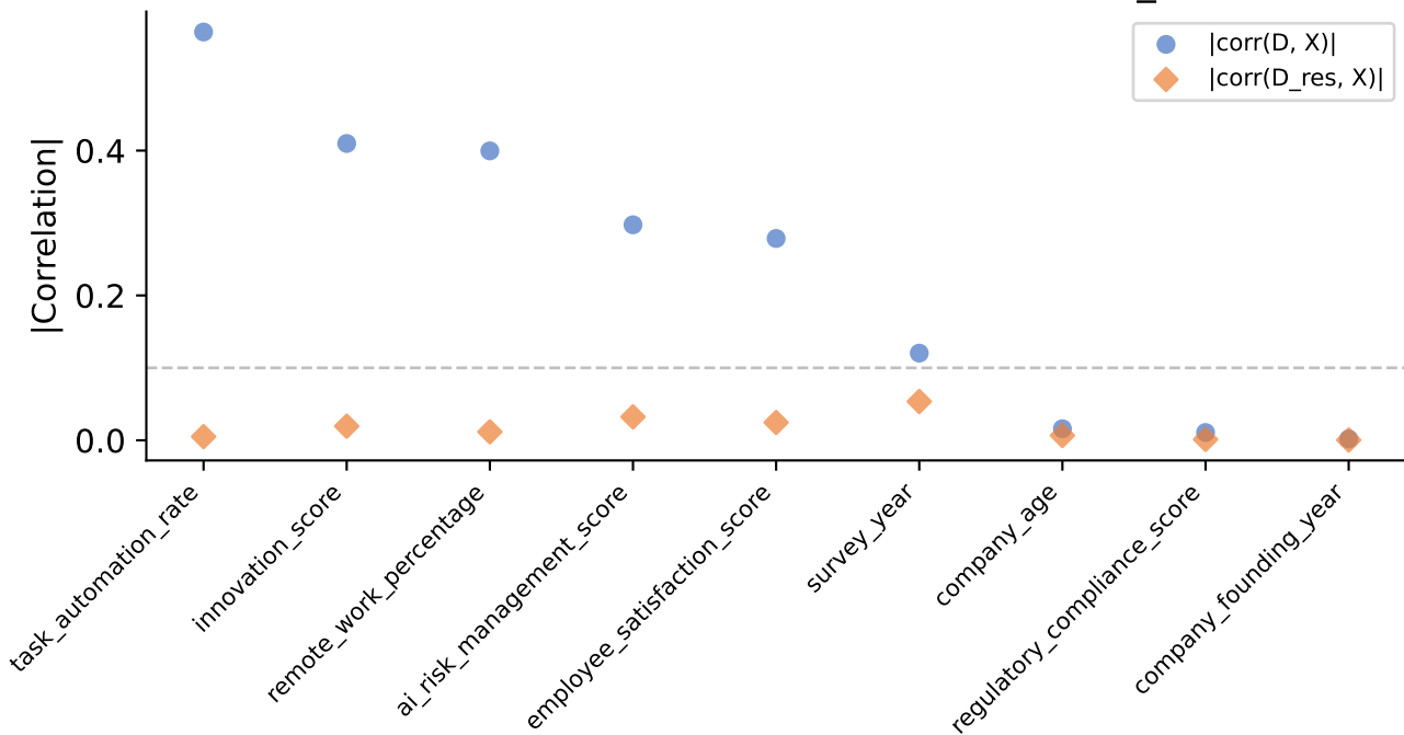
Covariate Balance (Correlation with D vs D_res)
