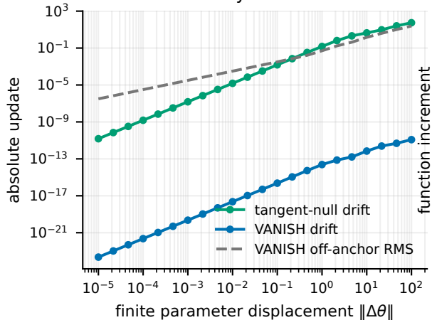
First-order safety fails at finite scale
