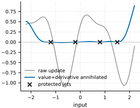
One operator protects values and slopes
