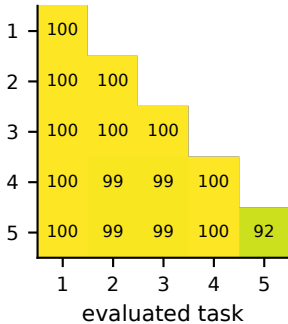
Functional L_2
