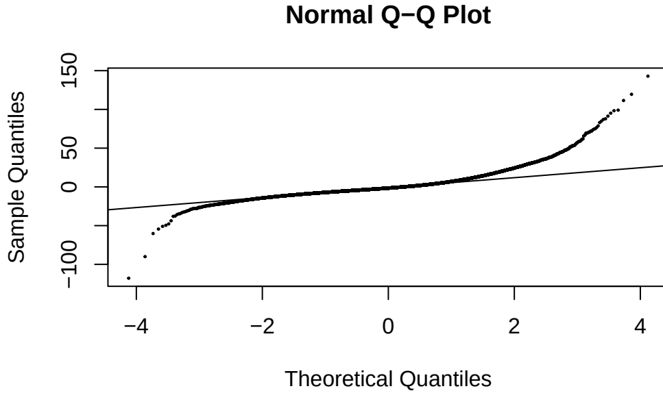
Figure 3: Normal Q-Q plot of the regression residuals. Points far from the reference line suggest problems with the normal-error assumption.
