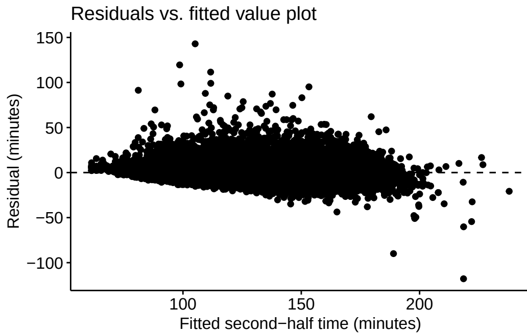
Figure 2: Residuals versus fitted second-half times, in minutes. The dashed line marks zero residual.
