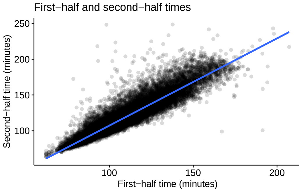
Figure 1: First-half and second-half times, in minutes, with the fitted regression line. Each point is one finisher.
