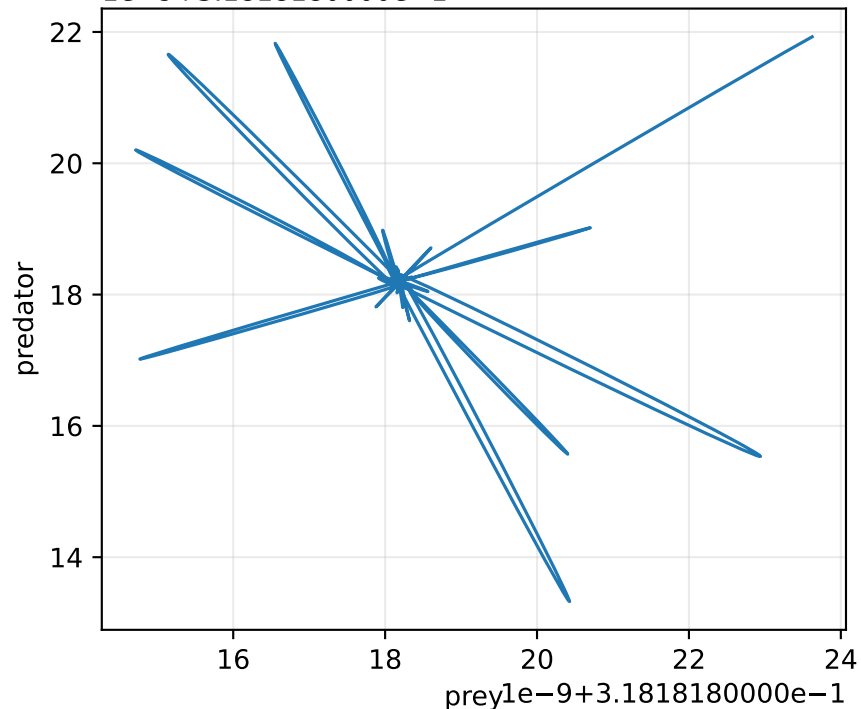
Leslie-Gower phase portrait
