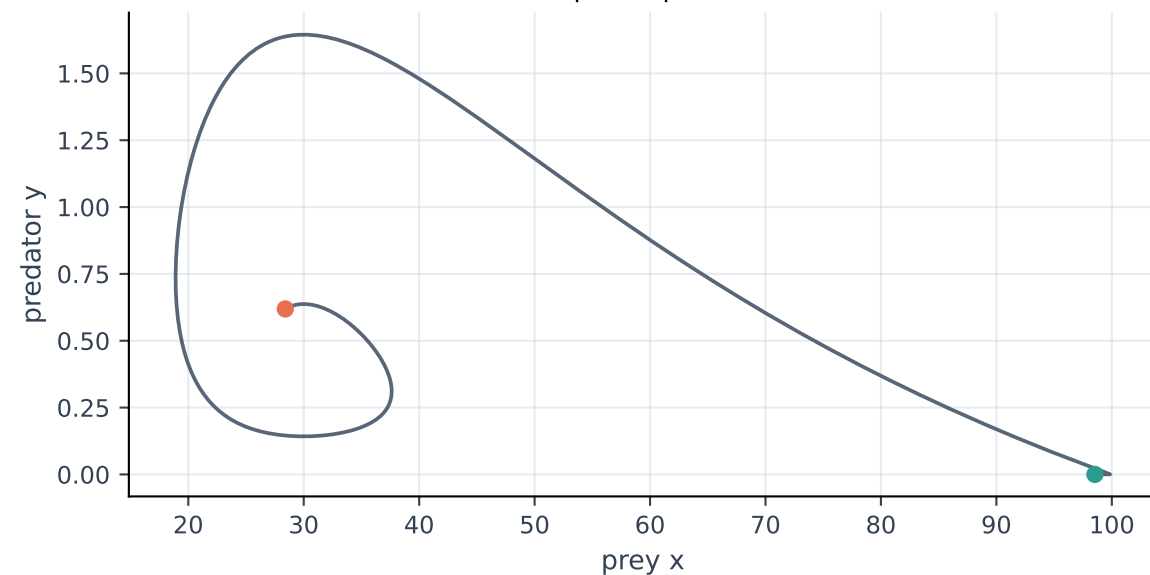
tail phase portrait
