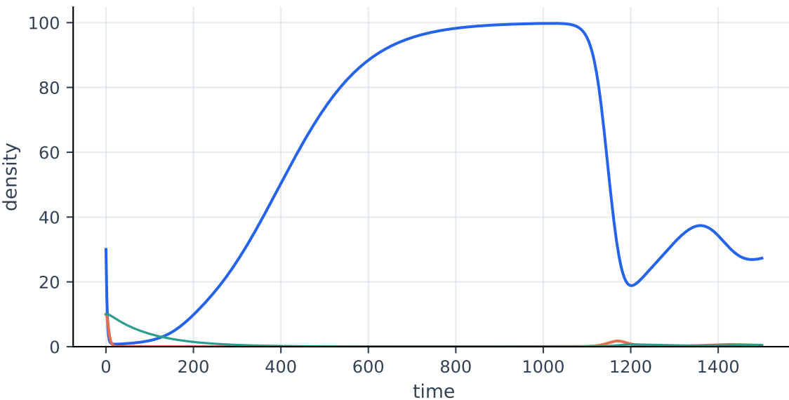
Case C: long memory amplifies oscillation: k=5.2 , \alpha=0.01
