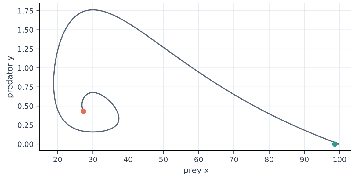
tail phase portrait
