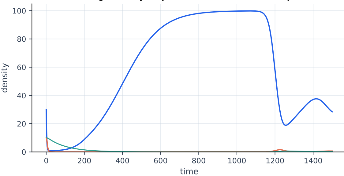
Case C: long memory amplifies oscillation: k=5.2 , \alpha=0.01
