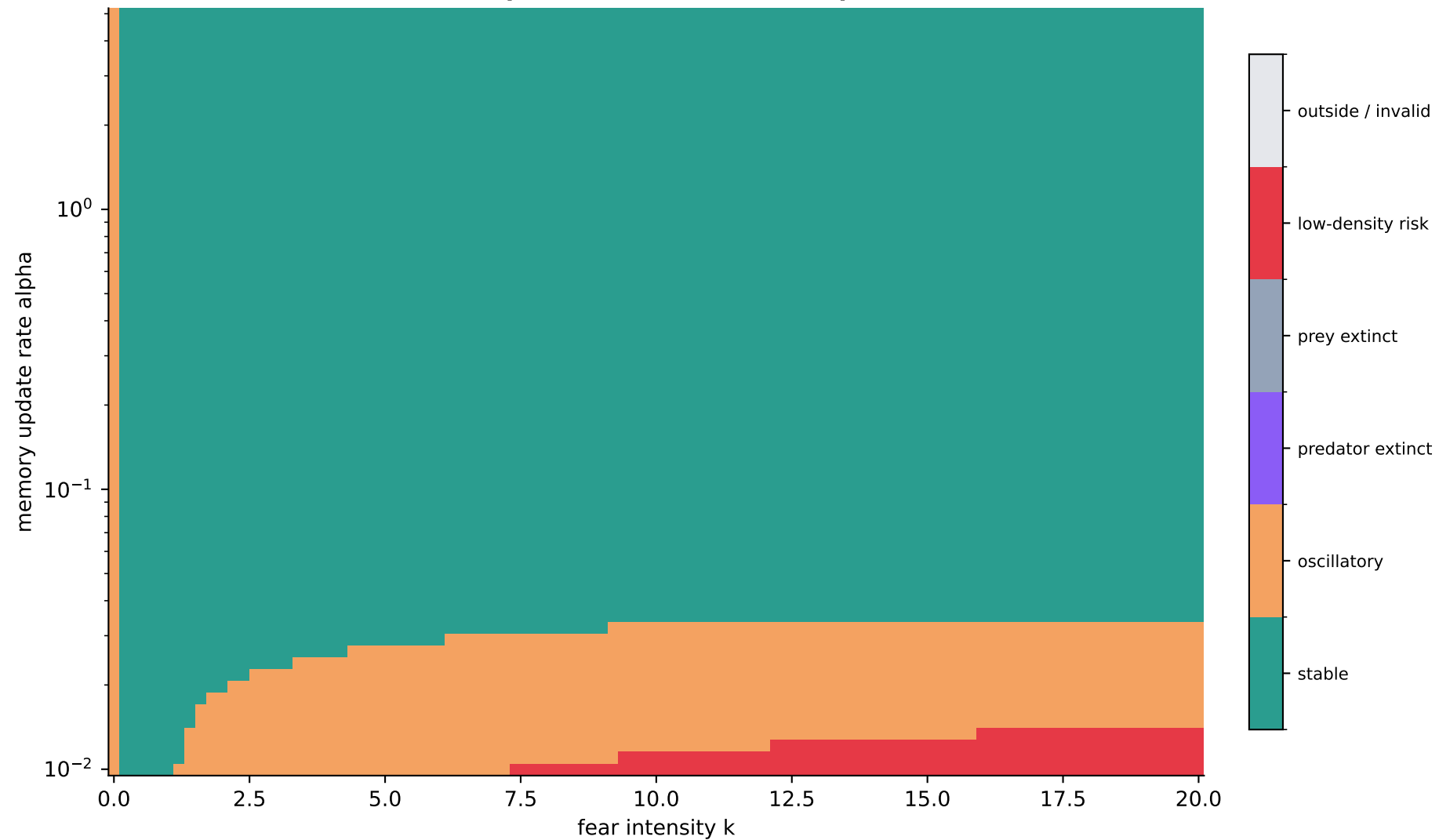
k-alpha classification heatmap
