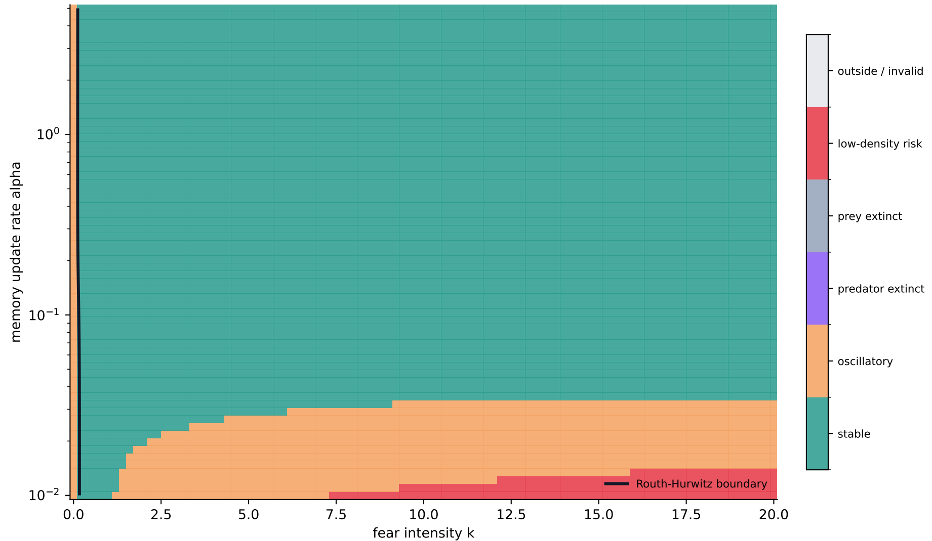
Routh-Hurwitz boundary over numerical classification
