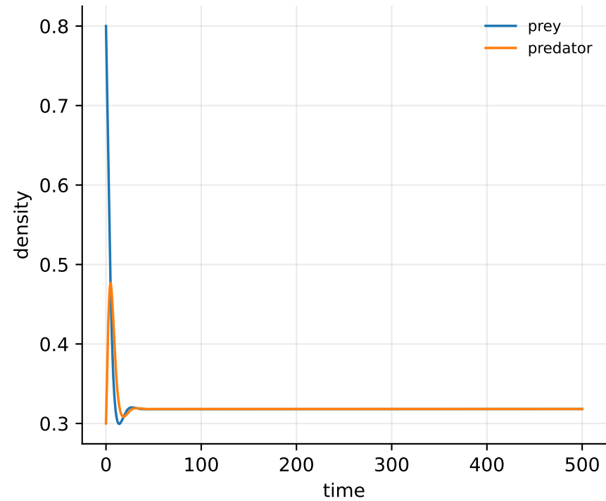
Leslie-Gower time series
