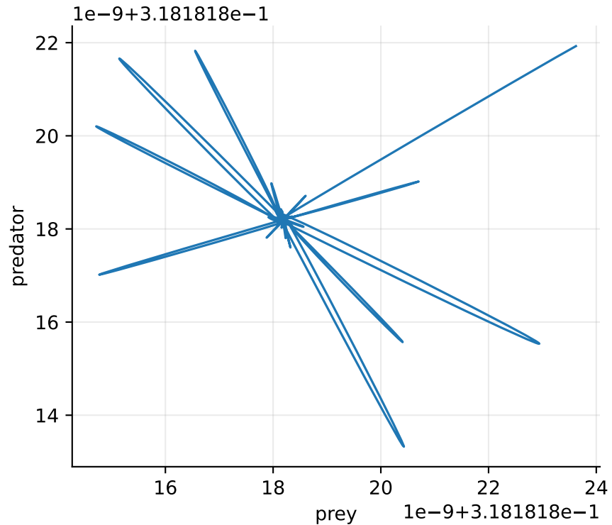
Leslie-Gower phase portrait
