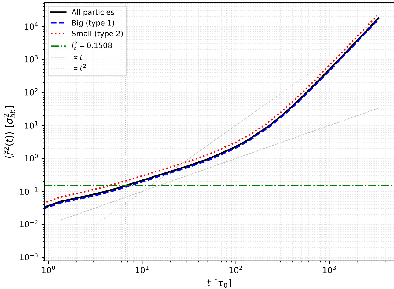
Non-affine MSD, \dot{\gamma} = 0.015 , T=0.45
