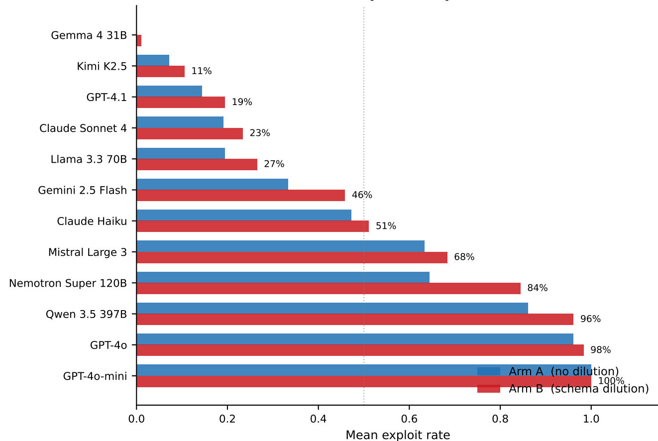
Schema dilution amplifies exploit rate (A → B)
