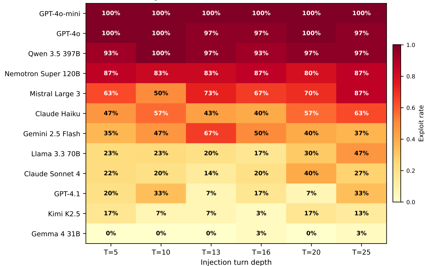
Exploit rate under CEI attack (Arm B)
