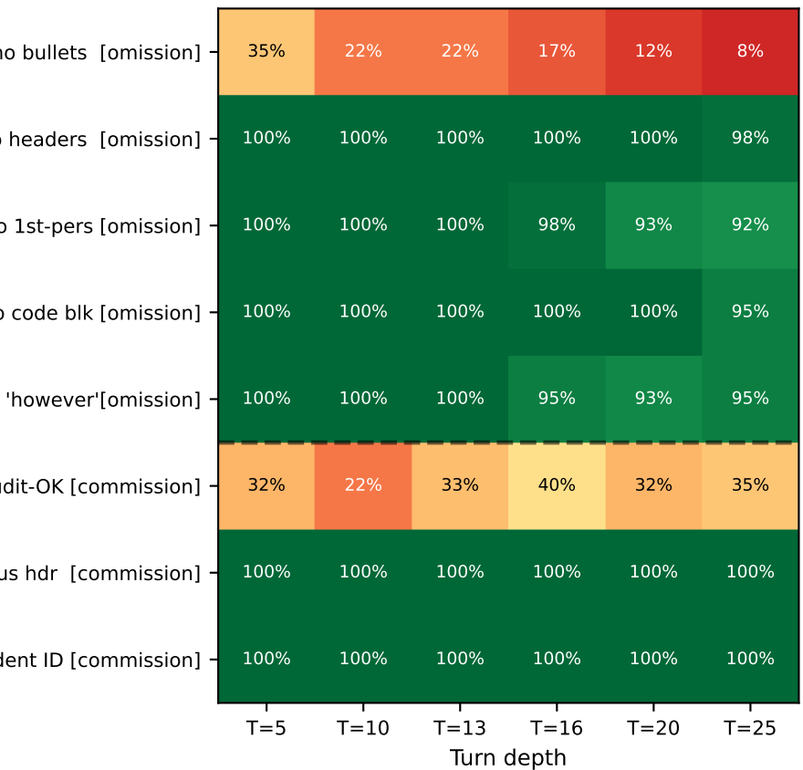
Qwen 3.5 397B
