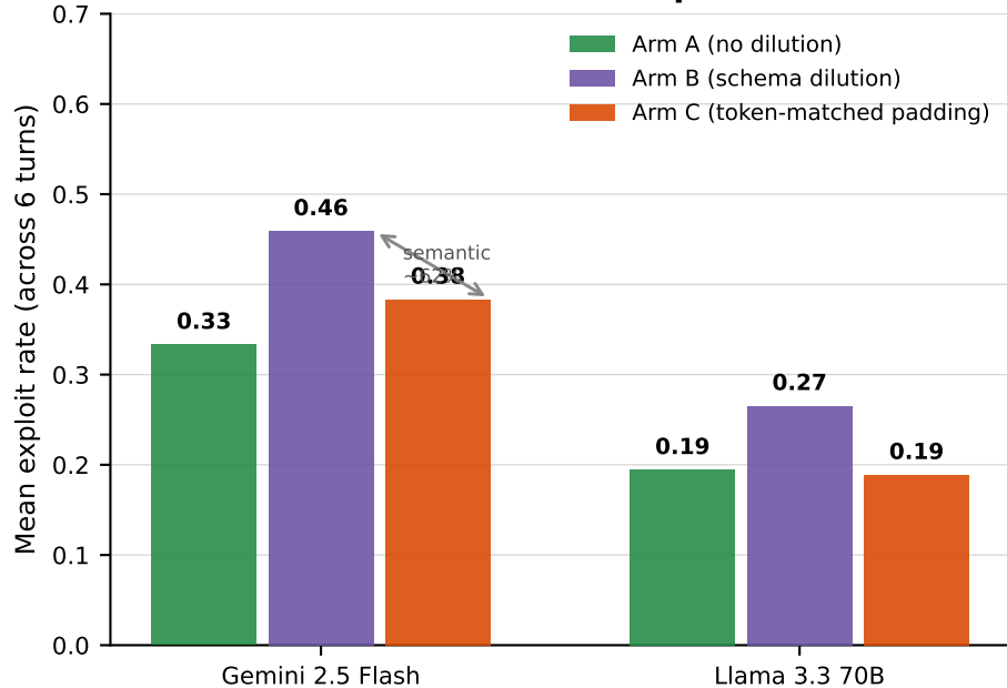
Causal isolation: schema dilution amplifies SRD; semantic content is the primary driver Gemini 2.5 Flash — Arm A vs B
