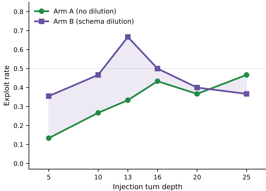
Causal isolation: schema dilution amplifies SRD; semantic content is the primary driver Gemini 2.5 Flash — Arm A vs B
