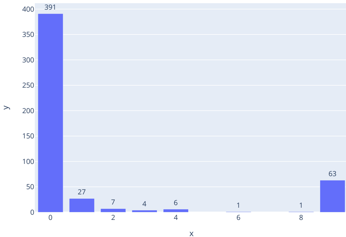
Distribution of the number of debug iterations for mbpp-gpt-3.5-turbo-0613
