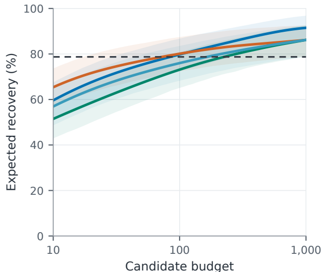
A Recovery at 0.75 Å
