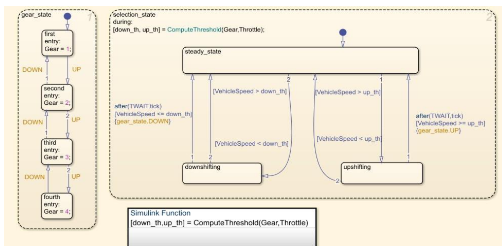
Figure 12 Shift logic Stateflow Diagram
