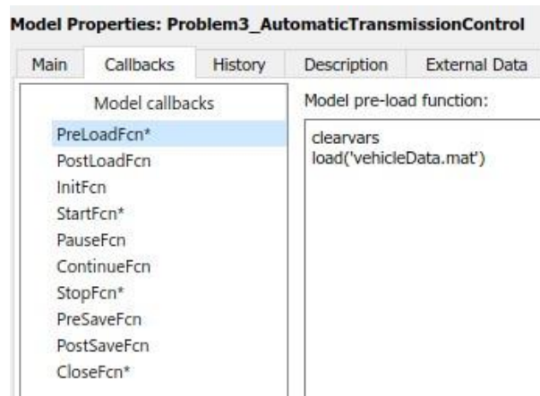
Figure 17 PreLoad Function
