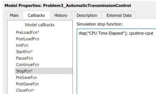
Figure 19 Stop Function
