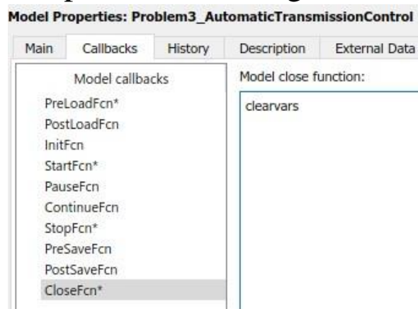
Figure 20 Close Function
