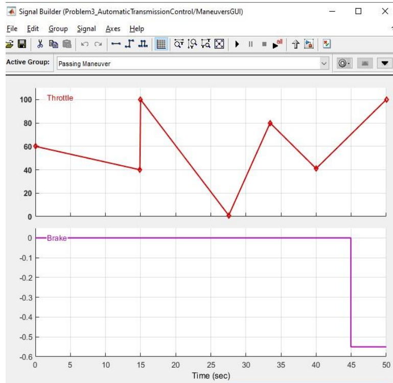
Figure 24 Signal Builder Implementation
