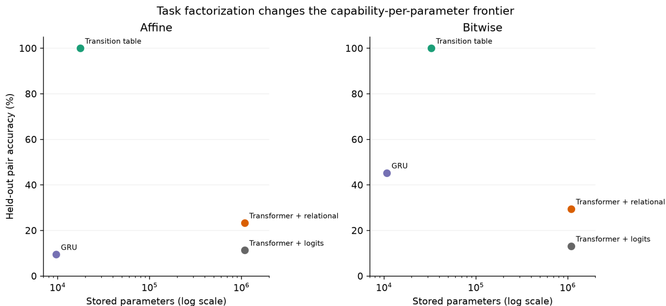
Figure 4. Held-out accuracy versus stored parameters. Task factorization moves the frontier far more than relational supervision. Bitwise values are descriptive only.
