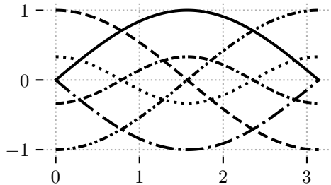
Figure 3.2: Linestyle
