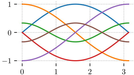
Figure 3.1: Colors
