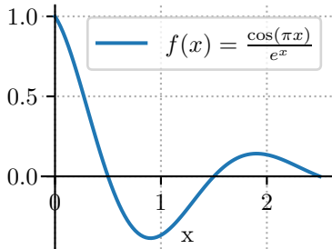
Figure 1.2: Spines through origin
