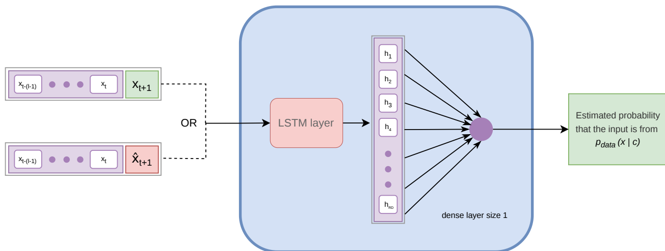
Discriminator D
