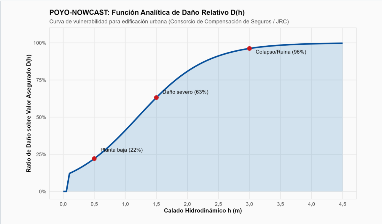
Figure 2: Analytical Relative Depth-Damage Vulnerability Function D(h). Empirical damage curve calibrated against CCS/JRC data for urban residential and commercial assets: Ground-floor damage threshold (22% at h=0.5m), Severe structural damage (63% at h=1.5m), and Structural Collapse/Ruin threshold (96% at h=3.0m).
