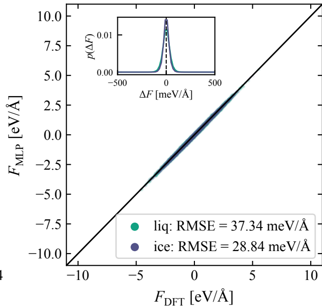
NEP: forces
