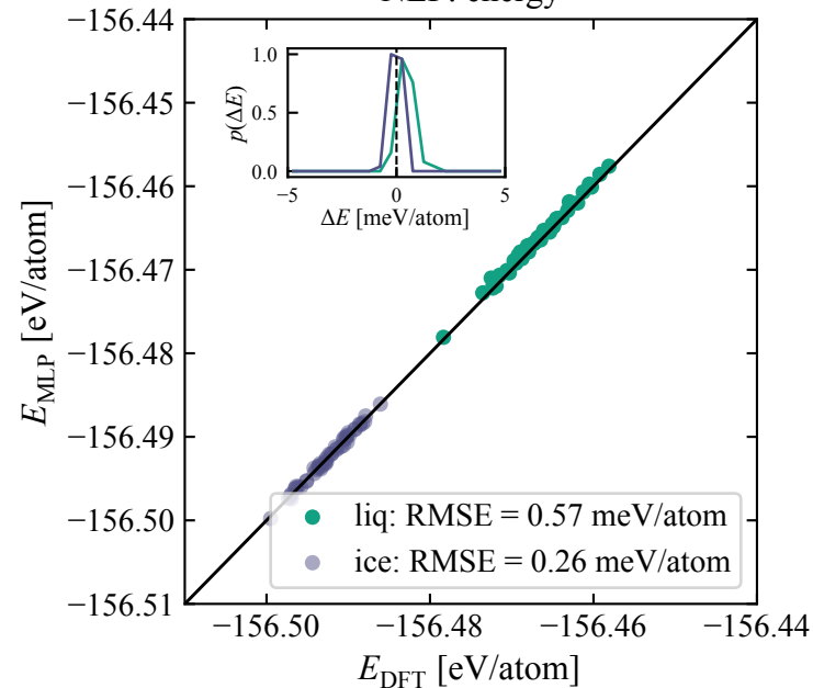
NEP: energy
