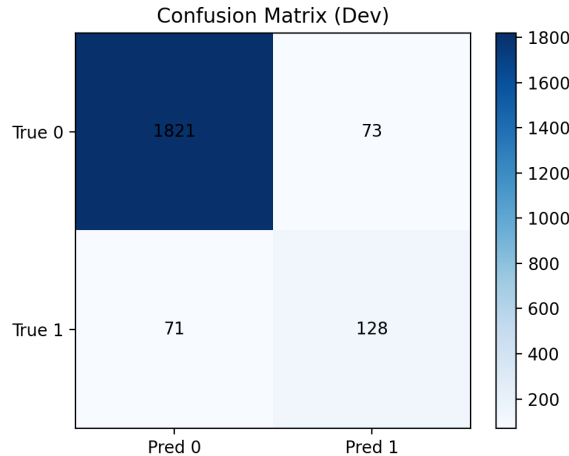
Figure 4: Confusion Matrix for TP/FP/FN/TN Trade-off
